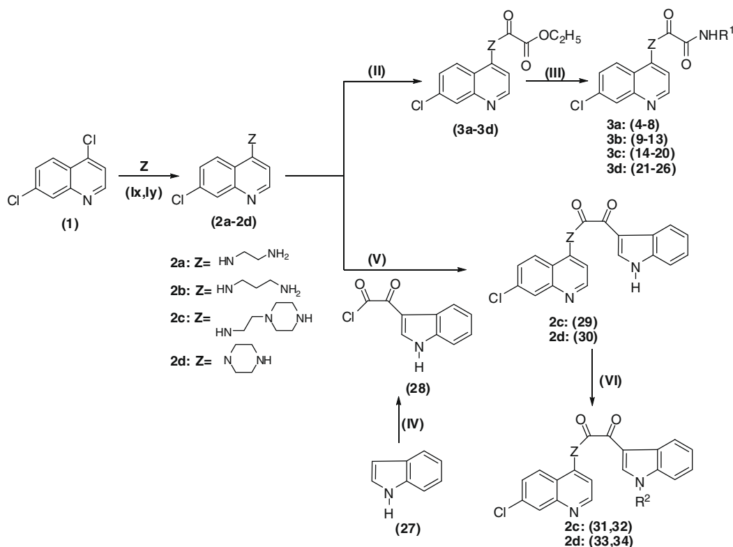
Scheme 1. Reagents and conditions: (I) (x) \alpha,\gamma -diamines, reflux, 7 h; (y) N -aminoethylpiperazine/piperazine, MeOH, reflux, 5 h; (II) ClCOCO2Et , DCM, rt, 1 h; (III) primary amines, n -BuOH, reflux under pressure, 8 h; (IV) (COCl)2 , dry Et2O , 0 °C, 1 h; (V) 2c/2d , Et3N , n -BuOH, reflux, 9 h; (VI) MeI/ PTSC, NaOH, TBAB, DCM, 0 °C–rt, 2 h.
