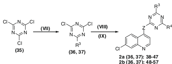
Scheme 2. Reagents and conditions: (VII) piperidine/morpholine, 0 °C, THF, 1 h; (VIII) 2a/2b , K2CO3 , THF, 4 h; (IX) different amines, K2CO3 , 80 °C, reflux, 6 h.
