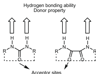
Figure 2. Hydrogen bonding ability of oxalamide group.
